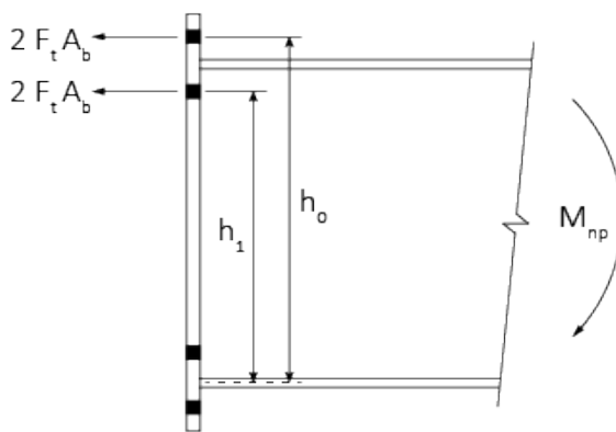
4 Bolt Configuration
