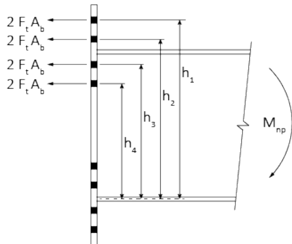
8 Bolt Configuration
