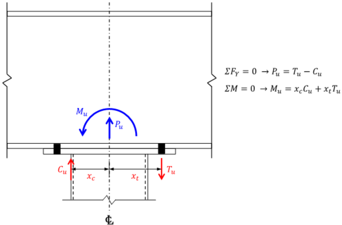
Beam Over HSS Connection Statics
