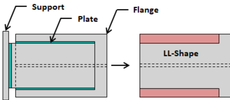
Block Shear Failure Modes – No End Weld & Plate Width < Flange Width
